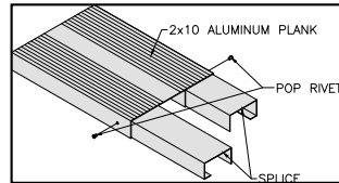
Plank Splice
