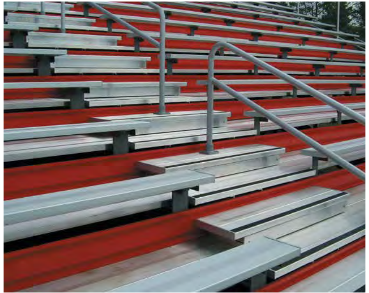
ALL OPENINGS CLOSED TO LESS THAN 4" FOR COMPLIANCE
