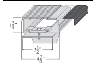
2" x 5" w/nosing
