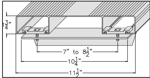
2" x 12"
