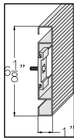
1" x 6"
