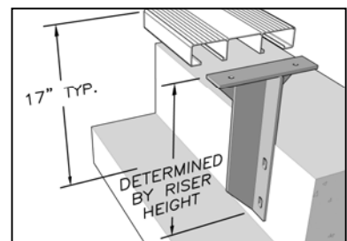
T Bracket
