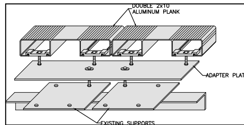
Double Foot Adapter Plate
