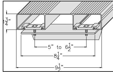
2" x 10"
