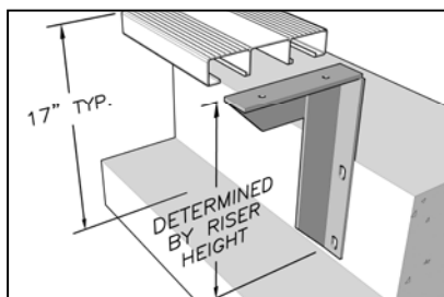
L Bracket
