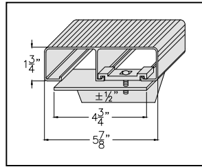
2" x 6"
