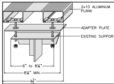
Seat Adapter Plate
