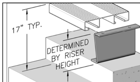
Z Bracket
